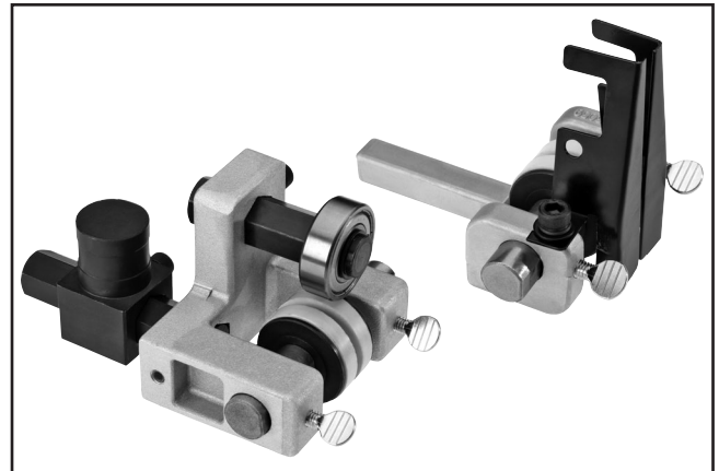
Figure 51. H7873 Ceramic Blade Guide Set.
